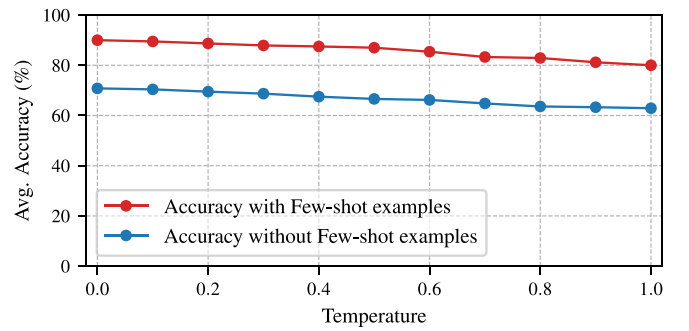
Fig. 10. Impact of sampling temperature in translating the generated dataset with and without Few-shot examples.
