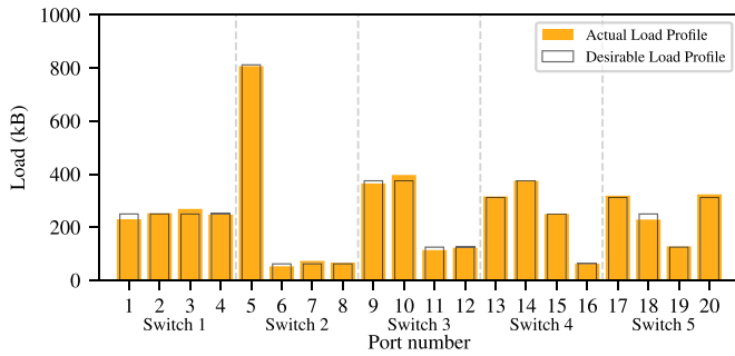
Fig. 9. Traffic follows the desired load profiling rule specified by the intent when installed directly on the data-plane.
